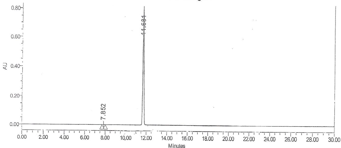
Auto-Scaled Chromatogram
